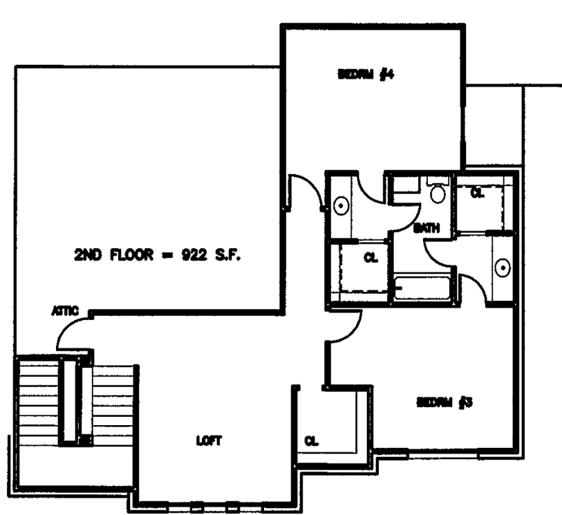
FLOOR PLAN
